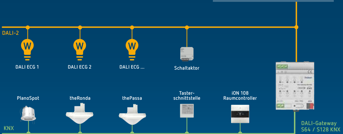
Systemschaubild: Single Master Application Controller
